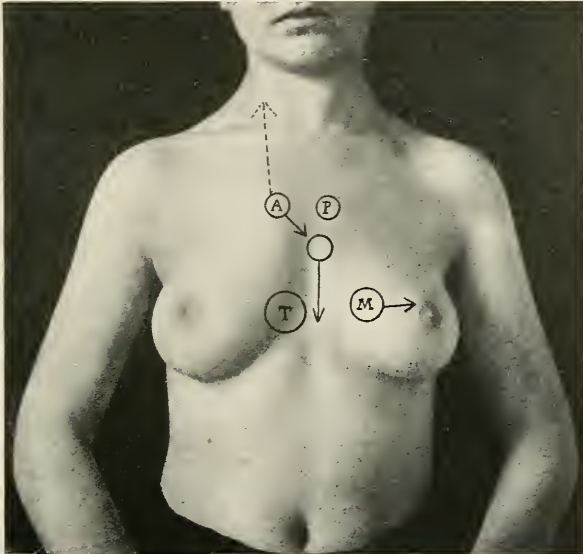
FIG. 178.—Showing the areas of the chest over which sounds produced at the various valvular orifices are generally most distinctly heard. A, aortic area; P, pulmonic area; M, mitral area; T, tricuspid area.
